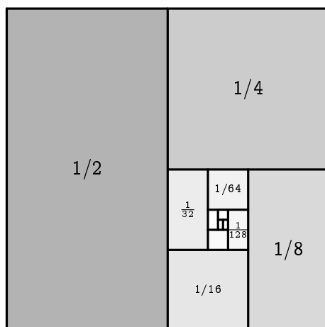
Figura 5.1: Series.
